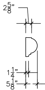
PROFILE M-75
