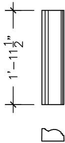
PROFILE M-60-S
