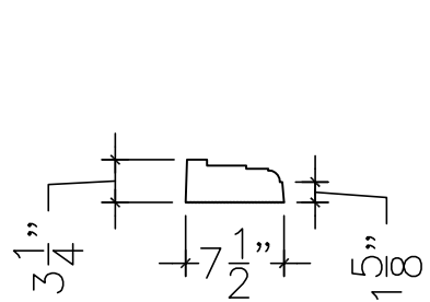
M-48 PROFILE
