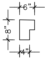
PROFILE M-73
