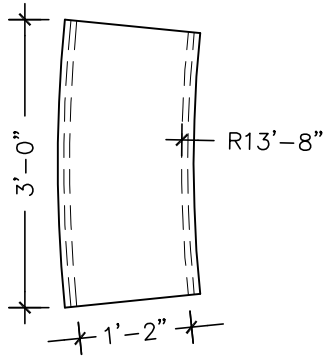
13'-8" RADIUS WC-8-13'8"RAD
