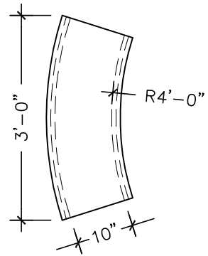
4' RAIUS WC-7-4'RAD
