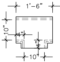
TEE WC-7-TEE
