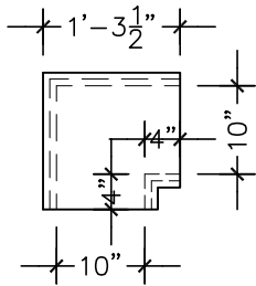
CORNER WC-7-C
